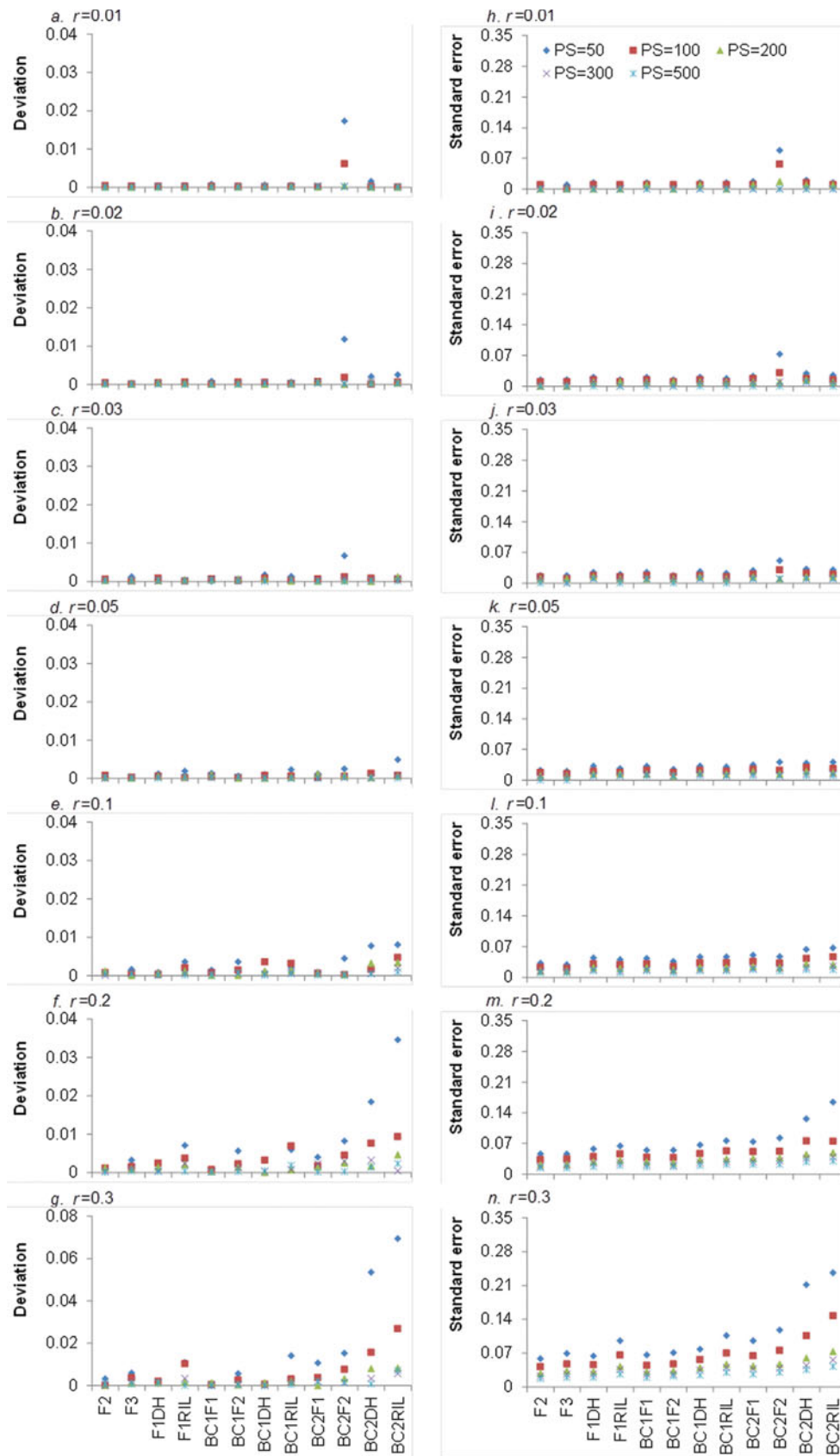
Fig. 3. Average deviations between estimated recombination frequencies and real recombination frequencies ( a–g ) and SEs of estimating recombination frequencies ( h–n ) from 1000 simulations in 12 bi-parental populations corresponding to seven levels of recombination frequencies ( r = 0.01, 0.02, 0.03, 0.05, 0.1, 0.2 and 0.3 ) and five PS (PS = 50, 100, 200, 300 and 500). Only co-dominant markers were considered.
